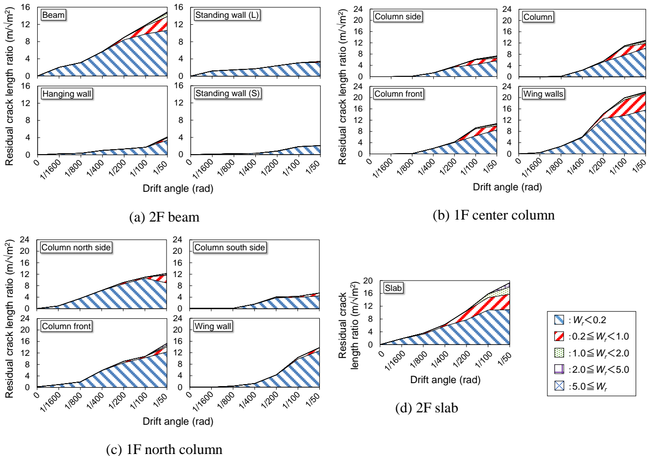
Fig. 4 – Residual crack length ratio
