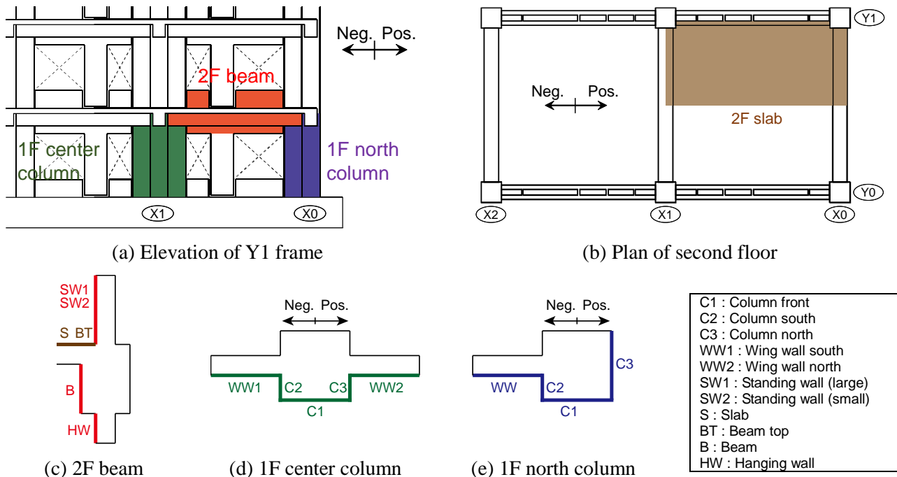
Fig. 1 – Regions for detail damage measurement
