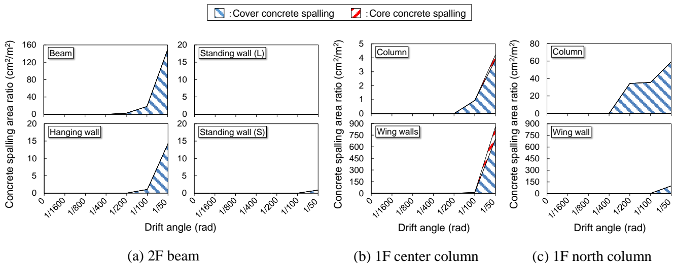
Fig. 5 – Concrete spalling area ratio
