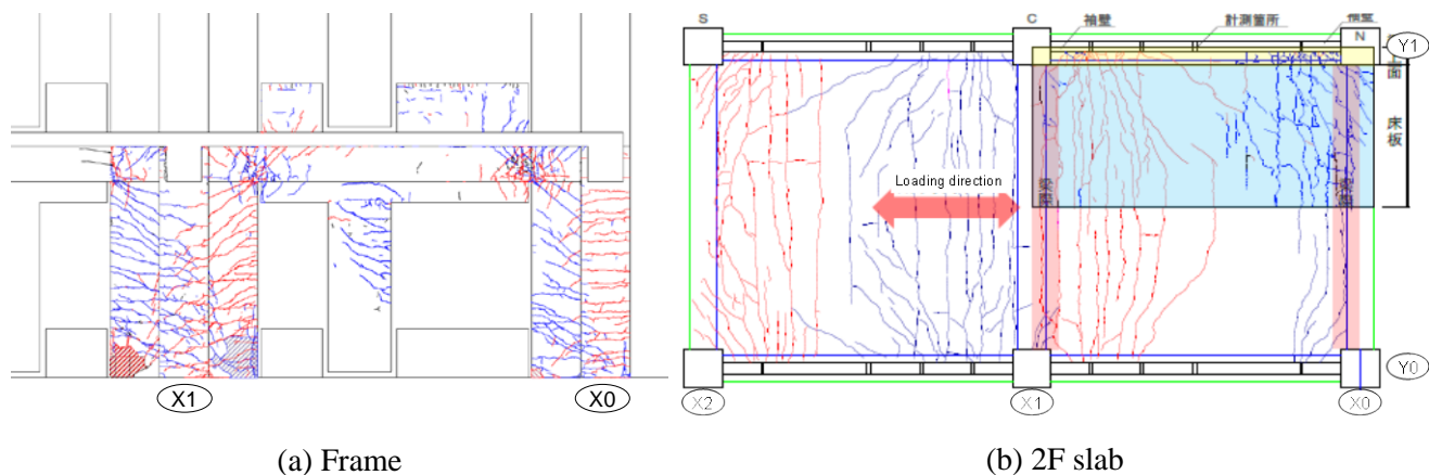
Fig. 2 – Residual crack diagram ( R=1/50 rad)
