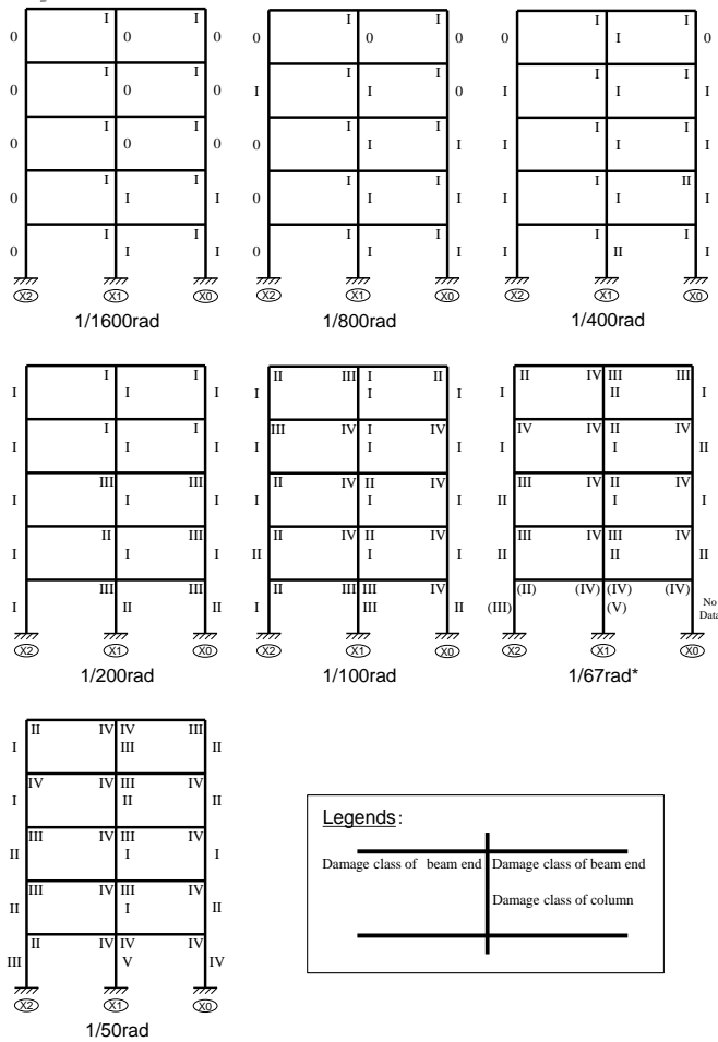
Fig. 6 – Damage class of each member
