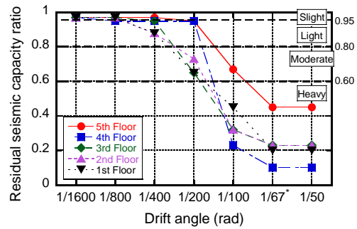
Fig. 7 – Residual seismic capacity ratio
