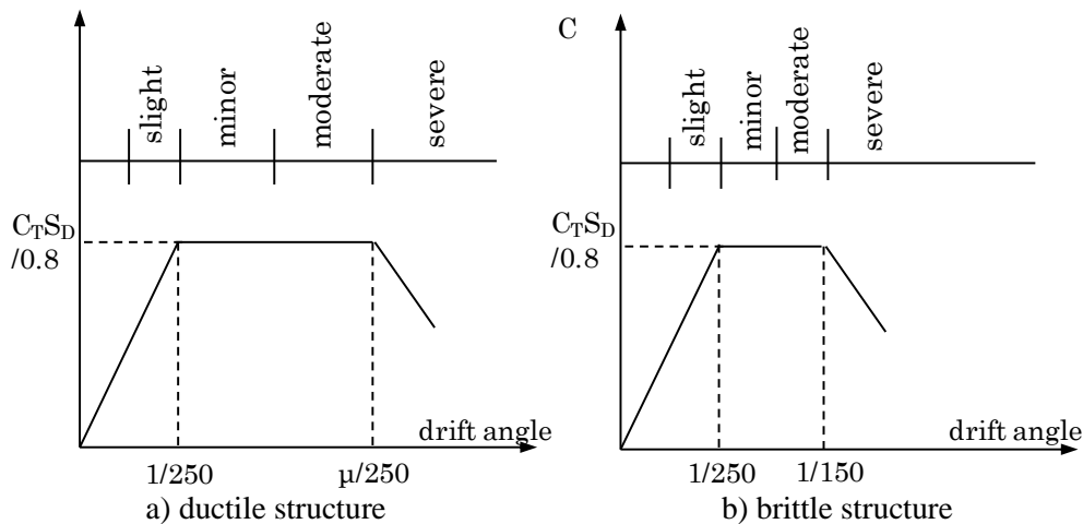
Figure 7 Base shear – lateral displacement relations and damage levels
