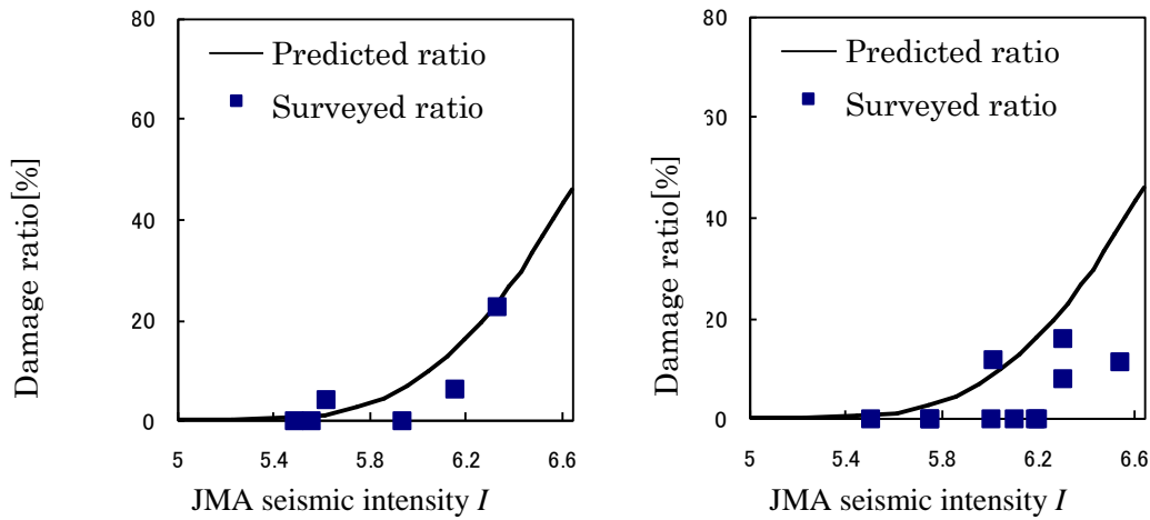
a) 2007 Notohantoh EQ b) 2007 Niigata-chuetsu-oki EQ Figure 9 JMA seismic intensity – damage ratio of timber houses
