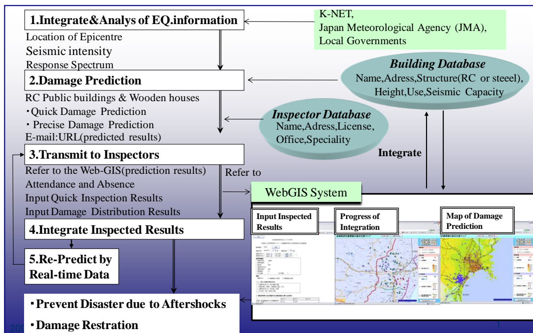
Figure 3 Flow of operation of the supporting system
