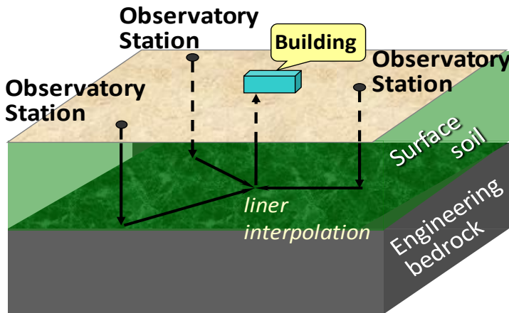
Figure 4 Concept of interpolation of seismic intensity
