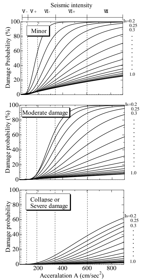
Figure 5 Fragility curve
