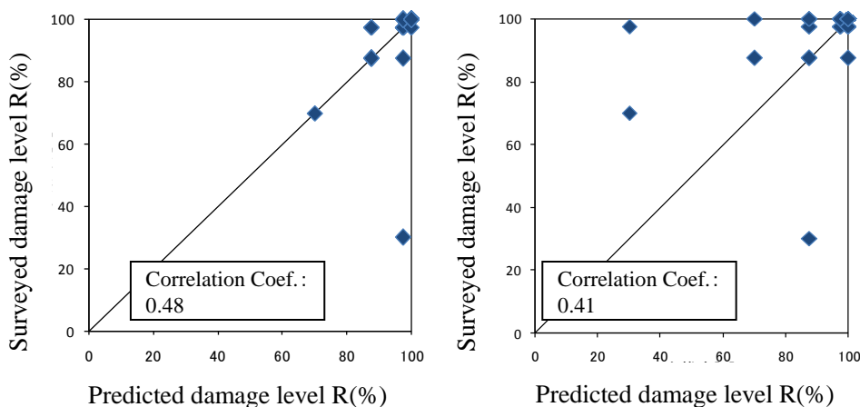
Figure 11 Comparison of observed damage ratio with predicted for RC buildings
