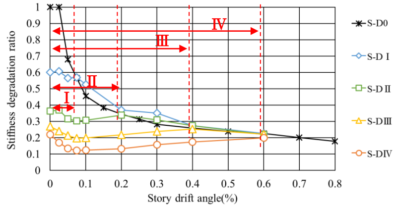
Fig.12–Stiffness degrading ratio
