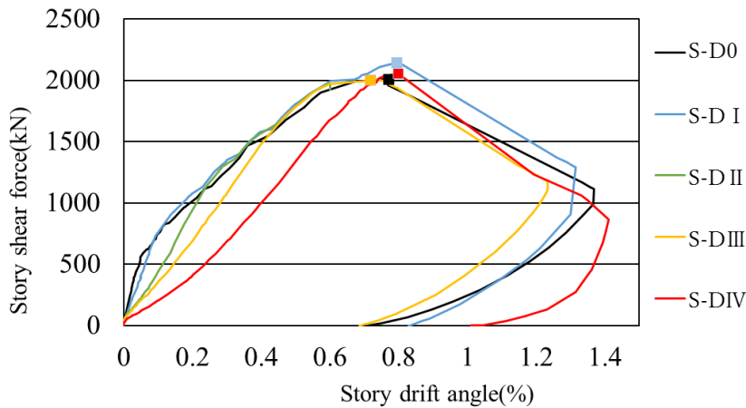
Fig.13(a) – Envelopes of shear-force – story drift curves with different levels of damage
