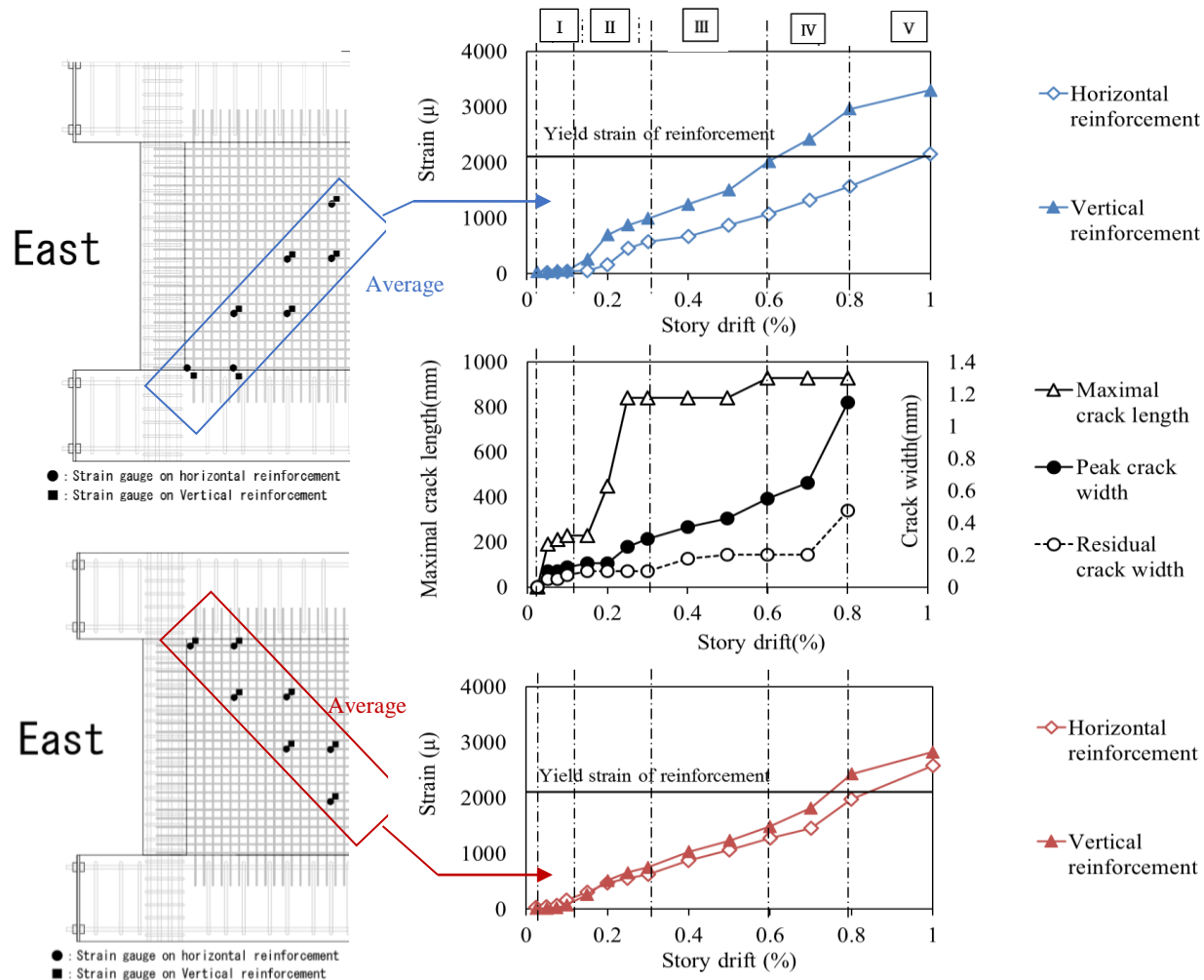
Fig. 8—Relationship between crack width/length and strain of reinforcement in wall panel
