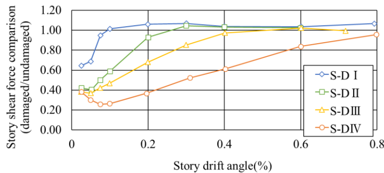
Fig.13(b)– Comparison of story shear force in each cycle
