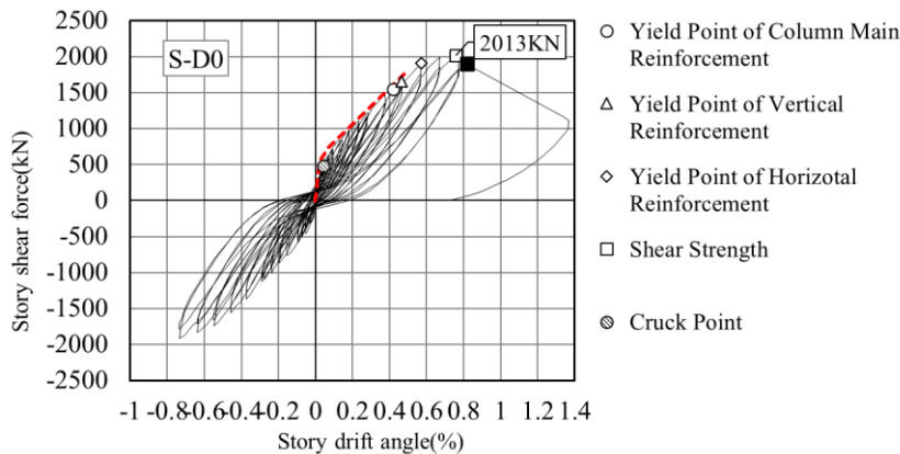
Fig. 4– Shear force-story drift angle relationship of S-D0
