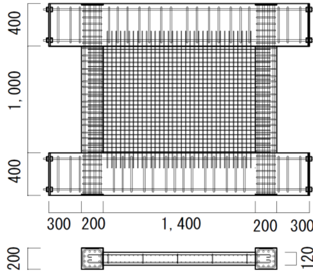
Fig. 1 – Reinforcing detail of specimen: elevation and section
