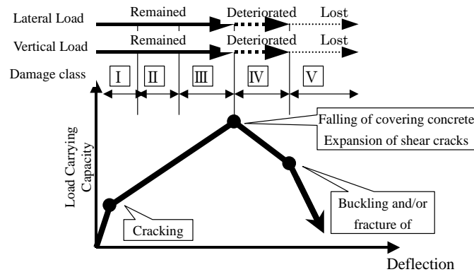
Fig. 7—Idealized lateral force-displacement relationships and damage class[2]
