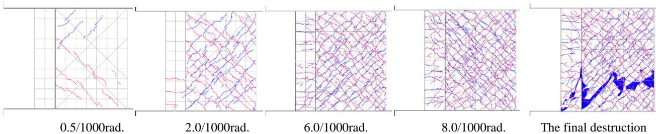
Fig. 6–Cracking maps of specimen S-D0
