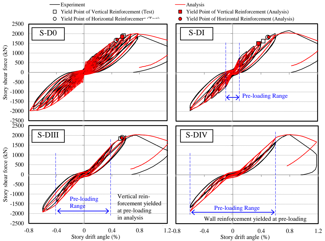
Fig.16 – Comparison of analysis and tests
