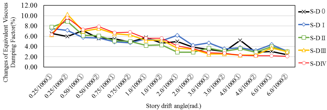
Fig.14– Equivalent viscous damping factor
