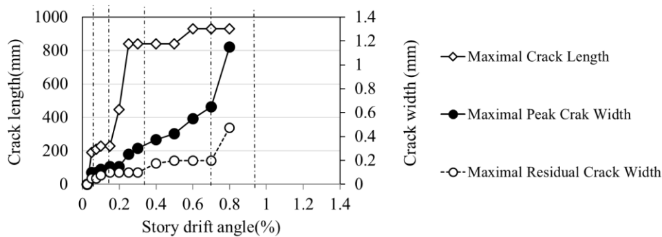
Fig. 9(b)–Damage class and crack width/length
