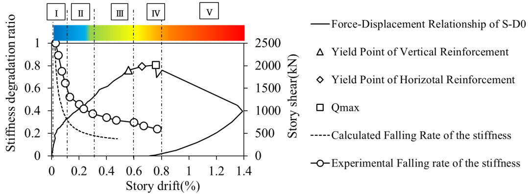
Fig. 9(a)–Damage class and stiffness degrading ratio
