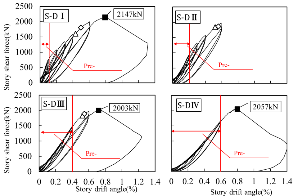
Fig.10–Shear force-story drift angle relationship of damaged specimens
