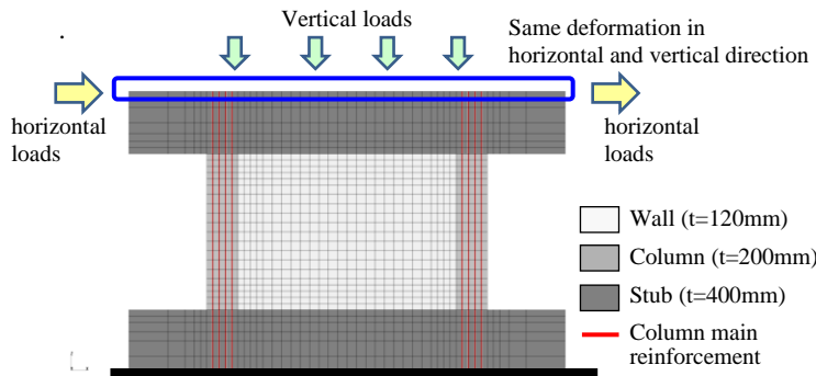
Fig.15 – Analytical model
