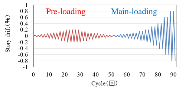
Fig.3-Loading history
