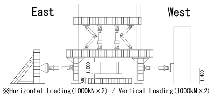
Fig.2 – Loading test setup
