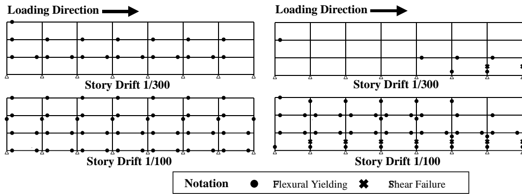
(a) Case1 (Uniaxial Bending Spring) (b) Case2 (MS Spring) Figure 12 : Location of Yield Hinge and Shear Failure in Y2 Frame
